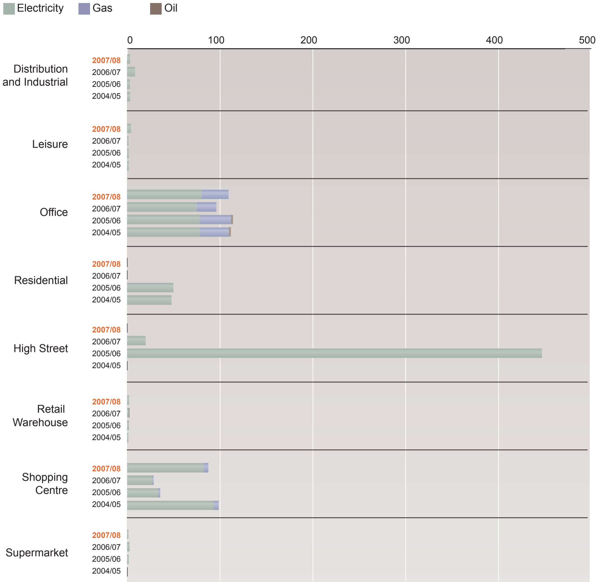
Figure 6: CO 2 emissions per property type (kg per m 2 )
