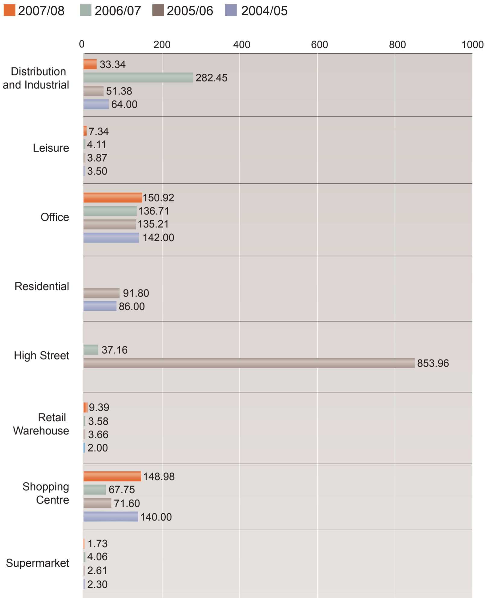
Figure 3: Average electricity consumption per property type (kWh/m 2 )
