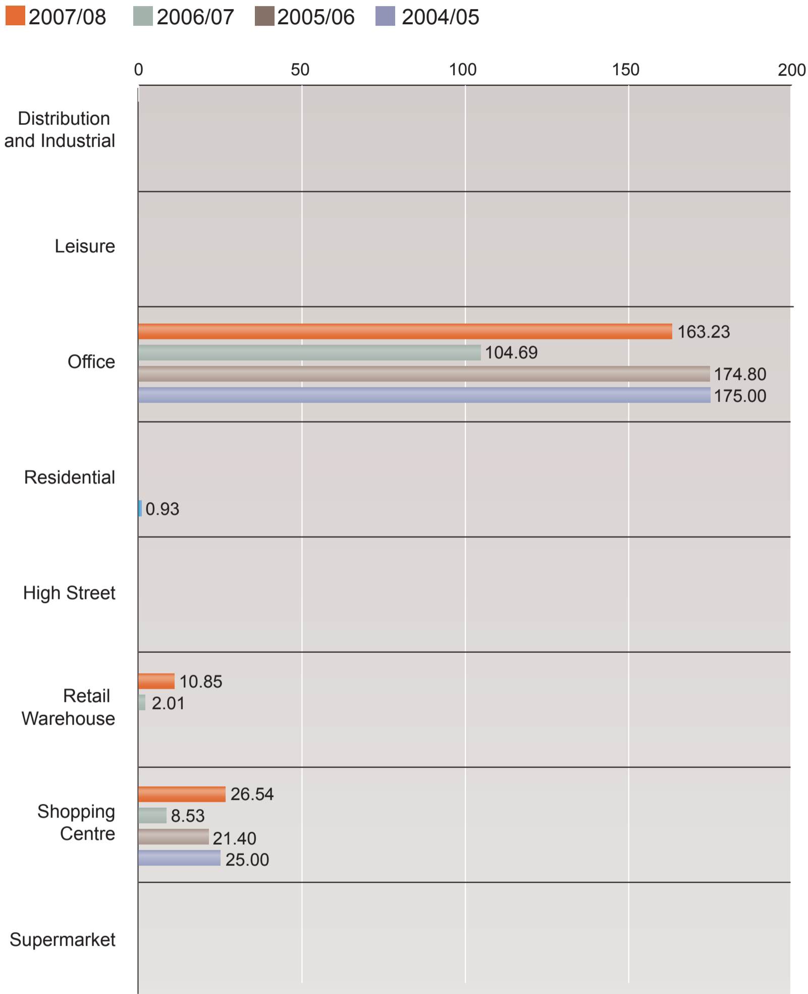
Figure 4: Average gas use per property type (kWh/m 2 )
